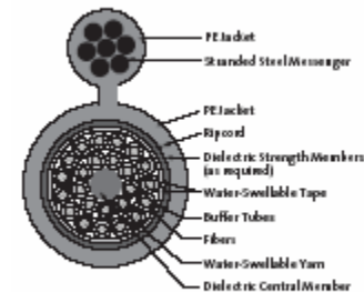
288-Fiber Single-Jacket Non-Armored Figure-8 ALTOS Cable | Drawing ZA-B14
