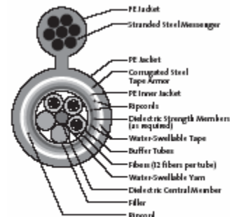
36-Fiber Double-Jacket Single-Armored Figure-8 ALTOS Cable | Drawing ZA-B15
