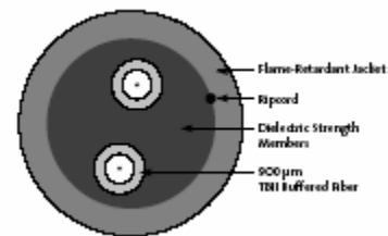
2-Fiber MIC Cable | Drawing CPC-220/V1/01
