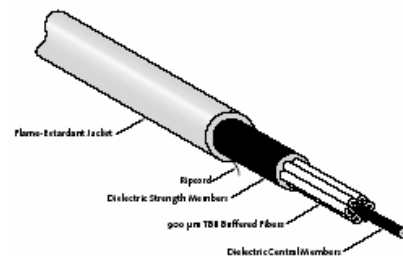
6-Fiber MIC Riser Cable | Drawing CPC-220/V1/03
