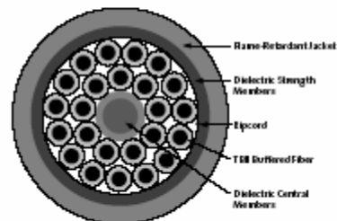
24-Fiber MIC Cable | Drawing CPC-220/V1/02
